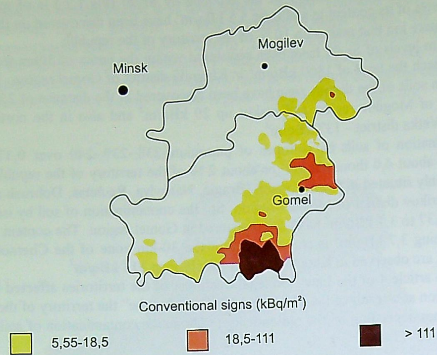
Fig. 1.7. Sr-90 content in soil on the territory of Gomel and Mogilev regions on 01.01.1995
